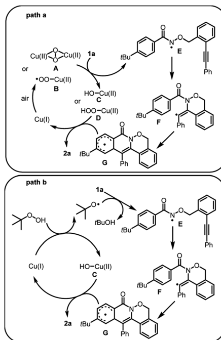
Scheme 1 Proposed mechanism.
