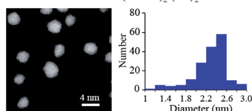
Fig. 4 Characterization of the non-covalent (Nb-E3) 2 ((K3) 2 AuNP assemblies. (A) Native PAGE analysis results to determine the average stoichiometry for the complete assembly of (Nb-E3) 2 with ((K3) 2 AuNPs. (B) Scanning transmission electron microscopy (STEM) analysis results of the (Nb-E3) 2 ((K3) 2 AuNP.
