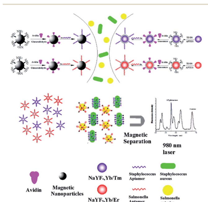
Fig. 26 Schematic illustration of the fabrication process of bio-functionalized UCNPs-MNPs and the working principle of the performed bioassay for the detection of Salmonella typhimurium and Staphylococcus aureus . Reprinted with permission from ref. 143. Copyright 2012, Elsevier B.V.
