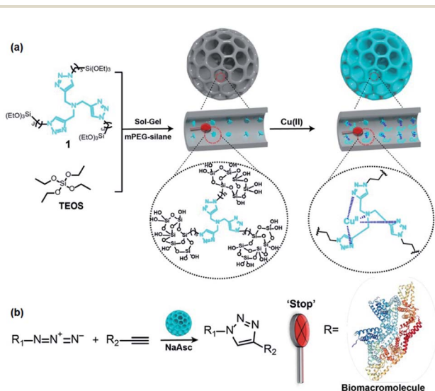
Fig. 45 (a) Cu-TTASi nanoreactors and the detailed coordination relations of Cu I and \text{N}(\text{C}_2\text{N}_3)_3 ligands and (b) Cu I -TTASi-catalyzed CuAAC reactions in the presence of sodium ascorbate. mPEG-silane: PEGylation triethoxysilane; NaAsc: sodium ascorbate. 235 Reproduced with permission. 235 Copyright 2021, American Chemical Society.
