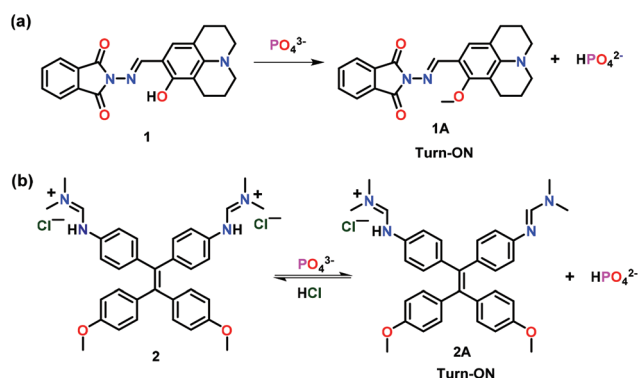
Fig. 1 Chemical drawings of chemosensors (a) 1 and (b) 2 and their proposed 'Turn-On' emission mechanism with \text{PO}_4^{3-} ions. Adapted from ref. 39 and 40.
