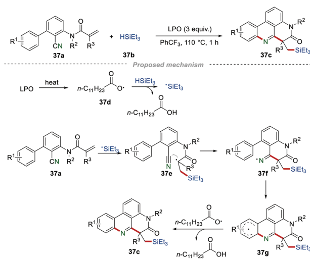
Scheme 37 The construction of silyl substituted phenanthridines.
