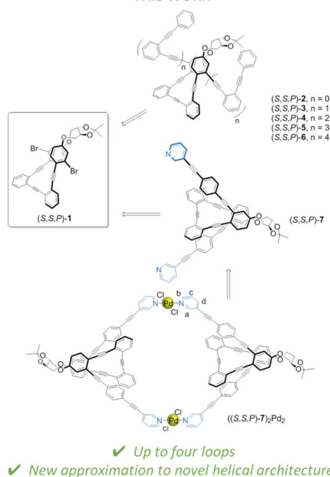
Fig. 1 Top: Previous studies with foldamers and helicene-type systems with more than two loops. Bottom: New helical systems developed in this work: chemical structure of stapled nucleus ( S,S,P )-1, helical systems ( S,S,P )-2–( S,S,P )-6, ligand ( S,S,P )-7 and metallosupramolecular complex (( S,S,P )-7) 2 Pd 2 .
