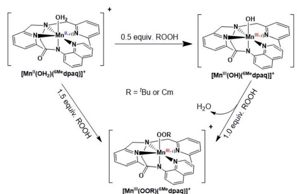
Scheme 1 Synthetic route for the preparation of [\text{Mn}^{\text{III}}(\text{OOR})(^6\text{Me dpag})]^+ .
