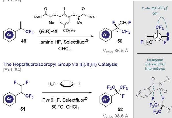
Fig. 12 Generating fluorinated surrogates of the isopropyl group via l )/ l (iii) catalysis.
