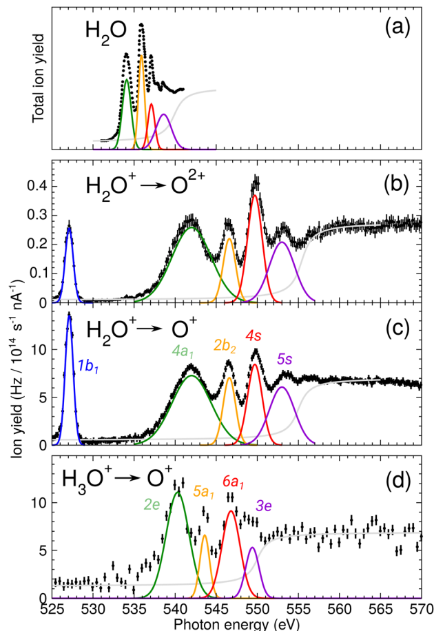
Fig. 3 (a) Total ion yield of neutral \text{H}_2\text{O} , digitized from the work of Piancastelli et al. , 27 (b) \text{H}_2\text{O}^+ \rightarrow \text{O}^{2+} , (c) \text{H}_2\text{O}^+ \rightarrow \text{O}^+ , and (d) \text{H}_3\text{O}^+ \rightarrow \text{O}^+ . The 1b_1 , 4a_1/3s , 2b_2/3p , 4s , and 5s resonance peaks have been fitted by Gaussians in blue, green, yellow, red, and purple, respectively. For \text{H}_3\text{O}^+ parent ions, the corresponding resonances have been fitted and are indicated in the same colors. An arc tangent function representing the ionization edge is plotted in grey for all channels. In panels (b)–(d), a constant background has been subtracted from the experimental data (see text).
