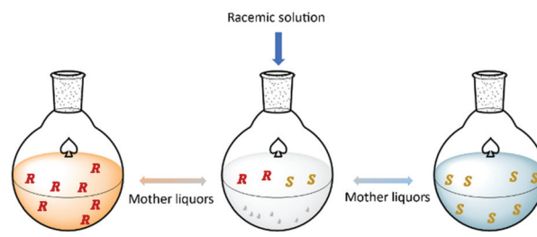
Fig. 6 Schematic illustration of coupled preferential crystallization using attrition. Adapted from ref. 93.
