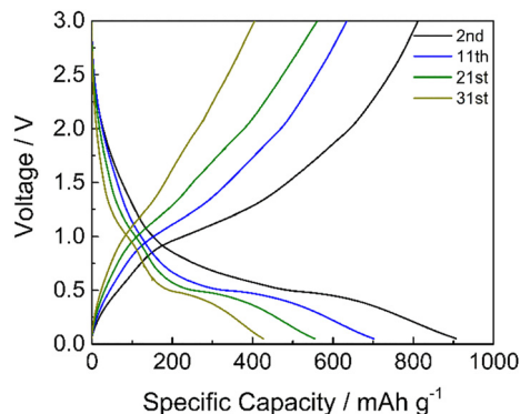
Fig. 10 GDC profiles of #3 in LP30 at 100 \text{ mA g}^{-1} .
