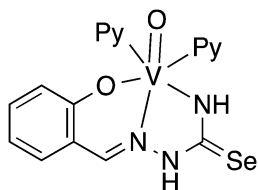
Fig. 10 Salicylaldehyde selenosemicarbazone as a dianionic [\text{O},\text{N},\text{N}]^{2-} ligand.
