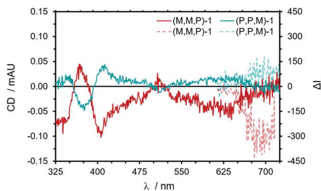
Fig. 4 Experimental ECD spectra of films of (M,M,P) -1 (red) and (P,P,M) -1 (turquoise) and experimental CPL spectra ( \lambda_{exc} = 370 nm) of (M,M,P) -1 (pale red, dotted) and (P,P,M) -1 (pale turquoise, dotted) on quartz substrates from CHCl_3 solutions at ca. 5 mg mL^{-1} .
