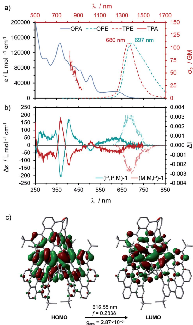
Fig. 3 (a) Experimental OPA (gray), OPE (turquoise, dashed), TPA (red) and TPE (red, dashed) spectra of (M,M,P/P,P,M) -1. Measured in CHCl_3 at ca. 1 \times 10^{-6} M, \lambda_{exc} = 370 nm for OPE, \lambda_{exc} = 900 nm for TPE; (b) experimental ECD spectra of (M,M,P) -1 (red) and (P,P,M) -1 (turquoise) measured in CHCl_3 at ca. 1 \times 10^{-6} M, and experimental CPL spectra ( \lambda_{exc} = 370 nm) of (M,M,P) -1 (pale red, dashed) and (P,P,M) -1 (pale turquoise, dashed) measured in CHCl_3 at ca. 1 \times 10^{-6} M; (c) HOMO and LUMO orbitals, and information of the TD-DFT calculated (CAM-B3LYP/6-31G(d,p)) lowest energy transition. The OPE spectrum is cropped at long wavelengths due to the use of a short path filter to block the multiphoton laser at the entrance of the photodetector.
