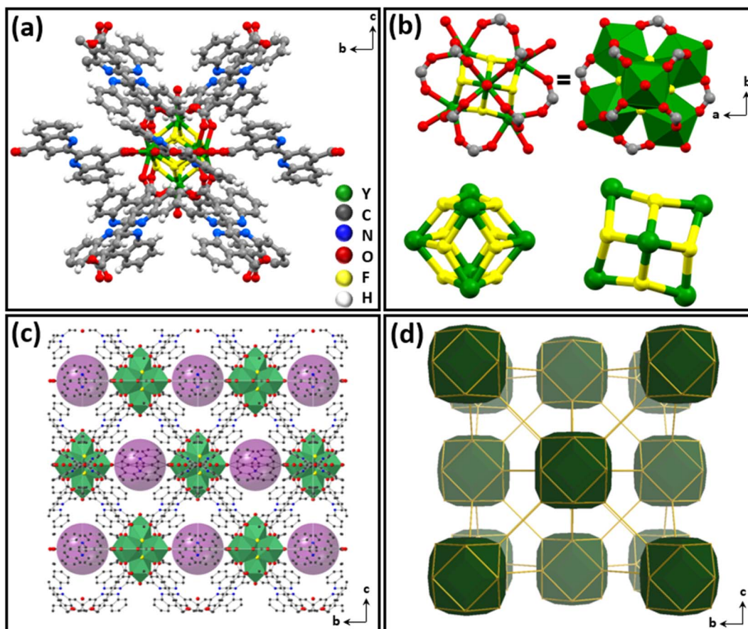
Fig. 4 Crystal structure of Y-BCA-3D (a) cluster structure with hexanuclear node, (b) c-axis view of hexacluster and isolated Y 6 F 8 cluster, (c) extended 3D network view along the a-axis showing 6.3 Å spherical cavities (purple), and (d) underlying net topology of the MOF viewed along the a-axis.
