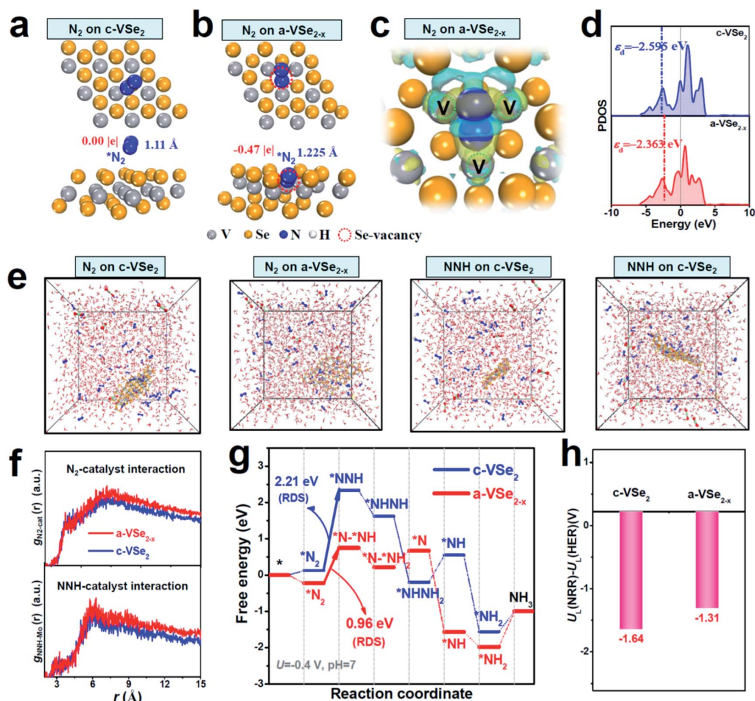
Fig. 4 (a and b) Optimized structures of N_2 on c-VSe 2 and a-VSe 2-x . (c) Electron deformation density of N_2 on a-VSe 2-x . Yellow and cyan isosurfaces represent electron accumulation and electron depletion, respectively. (d) PDOS of V-3d in c-VSe 2 and a-VSe 2-x for determining the d-band center ( \epsilon_d ). (e) Snapshots of the dynamic process of N_2 /NNH adsorption on c-VSe 2 and a-VSe 2-x in LiClO 4 electrolyte after 5 ns MD simulations, and corresponding (f) RDF curves of N_2 -catalyst and NNH-catalyst interactions. (g) Free energy diagrams of energetically favorable NRR pathways on c-VSe 2 and a-VSe 2-x at U = -0.4 V and pH = 7. (h) U_L(\text{NRR}) - U_L(\text{HER}) of c-VSe 2 and a-VSe 2-x .
