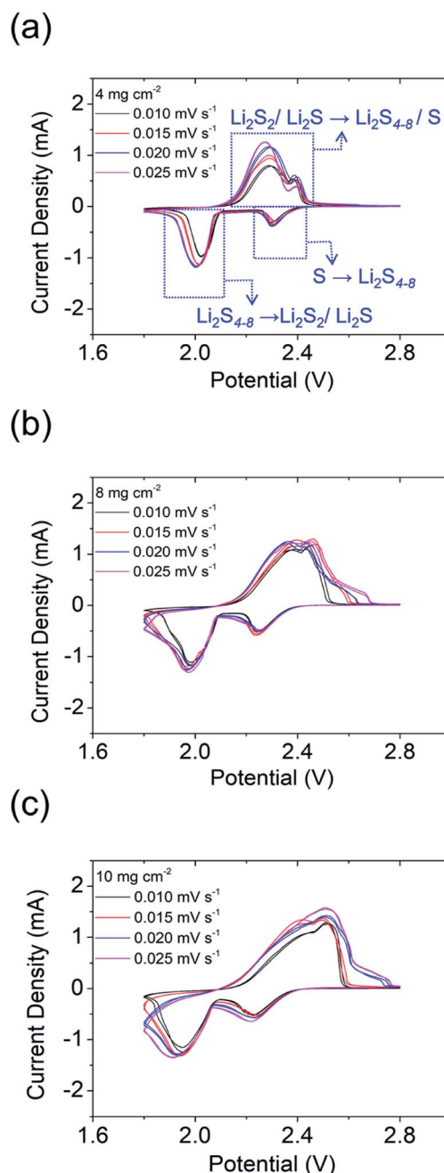
Fig. 4 Cyclic voltammograms of high-sulfur-loading cells: (a) 4 mg cm -2 ; (b) 8 mg cm -2 ; (c) 10 mg cm -2 .
