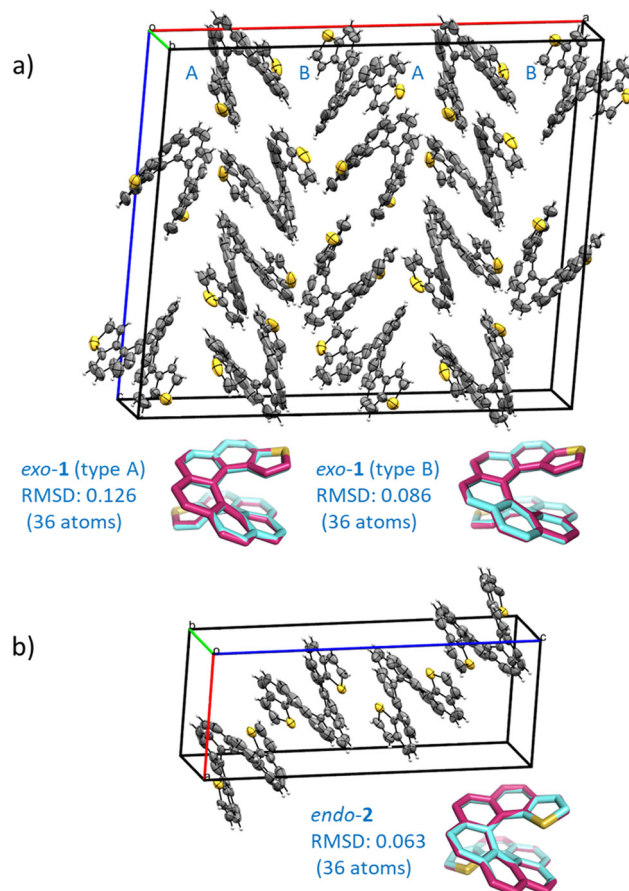
Fig. 1 (a) Crystal structure of the racemate exo -dithia[9]helicene (1): Monoclinic unit cell, space group C2/c , a = 33.075(4) , b = 9.8984(11) , c = 28.178(3) \text{ \AA} ; \alpha = 90^\circ , \beta = 94.890(2)^\circ , \gamma = 90^\circ ; Z = 16 ; CCDC number 2184340. The experimental structures of both molecular types found in the unit cell (A and B, reported in cyan) are overlapped with the calculated CAM-B3LYP/def2-SV(P) structures (in magenta) and shown below the unit cell; (b) crystal structure of the racemate endo -dithia[9]helicene-2: Monoclinic unit cell, space group P2_1/n , a = 9.712(2) , b = 9.709(3) , c = 25.072(6) \text{ \AA} ; \alpha = 90^\circ , \beta = 94.401(7)^\circ , \gamma = 90^\circ ; Z = 4 ; CCDC number 2184341. The experimental and calculated (CAM-B3LYP/def2-SV(P)) structures, reported in cyan and magenta respectively, are overlapped and shown below the unit cell. The root mean square deviation (RMSD, in \text{\AA} ) is calculated considering only the heavy atoms of an isolated dithia[9]helicene of ( M ) configuration for both isomers. For the crystal cells, ORTEP diagrams are shown with thermal ellipsoids drawn at 50% probability. The data was acquired at room temperature.
