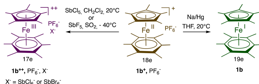
Scheme 3 Synthesis of the stable, fully methylated mixed sandwich Fe complexes with 17 and 19 valence electrons [ d^5 , \text{Fe(III)} resp. d^7 , \text{Fe(I)} ] that are both redox catalysts and electrocatalysts.
