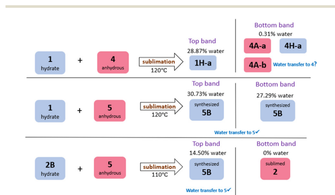
Fig. 3 Summary of results from competition experiments based on 1:1 mole-ratio co-sublimations.
