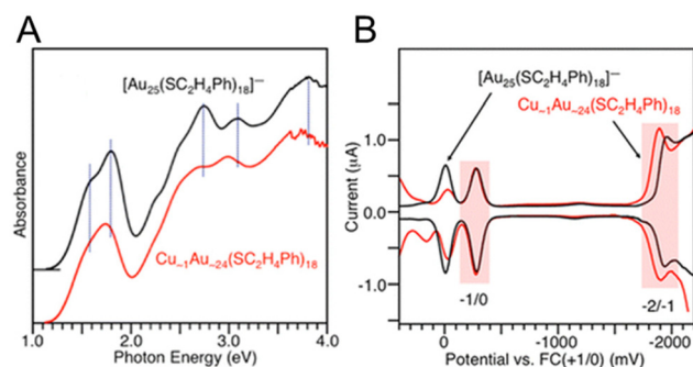
Fig. 10 (A) Optical absorption spectra of \text{Cu}_{1.1}\text{Au}_{24.1}(\text{PET})_{18} and [\text{Au}_{25}(\text{PET})_{18}]^- . The dotted lines indicate the main peak positions in the absorption spectrum of [\text{Au}_{25}(\text{PET})_{18}]^- . (B) DPV curves of \text{Cu}_{1.1}\text{Au}_{24.1}(\text{PET})_{18} and [\text{Au}_{25}(\text{PET})_{18}]^- . The red shaded regions indicate the peaks derived from the redox potentials of -2/-1 and -1/0 . Reproduced with permission from ref. 111. Copyright 2012, American Chemical Society.
