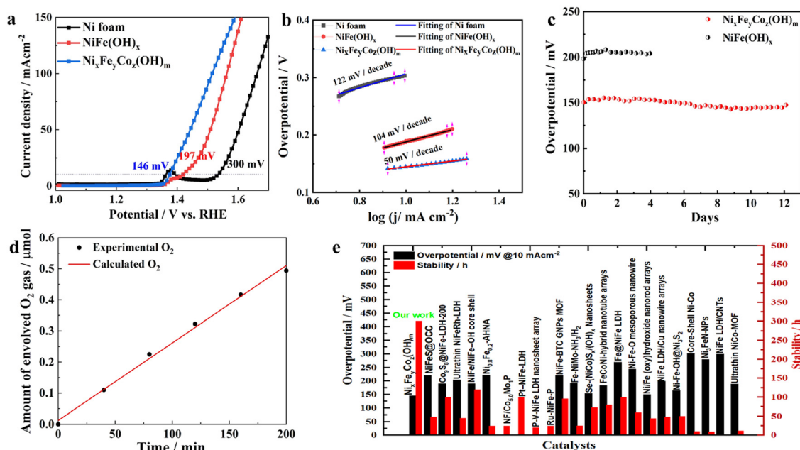
Fig. 2 OER performance. (a) Polarization curves after IR-compensation and (b) corresponding Tafel plots of the NF, \text{NiFe}(\text{OH})_x , and \text{Ni}_x\text{Fe}_y\text{Co}_z(\text{OH})_m electrodes in 1 M KOH. (c) Long-term stability tests at a constant current density of 10 \text{mA cm}^{-2} for the \text{NiFe}(\text{OH})_x , and \text{Ni}_x\text{Fe}_y\text{Co}_z(\text{OH})_m electrodes in 1 M KOH. (d) \text{O}_2 amounts detected by gas chromatography (dark dots) and the calculated amounts of \text{O}_2 (red line) by \text{Ni}_x\text{Fe}_y\text{Co}_z(\text{OH})_m catalyst. The measurement was performed at j_{\text{OER}} = 10 \text{ mA cm}^{-2} in 1 M KOH. (e) Comparison of this work and reported overpotential required to achieve current densities of 10 \text{mA cm}^{-2} and the related stability for various catalysts in 1 M KOH. RHE stands for reversible hydrogen electrode.
