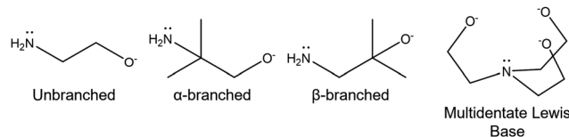
Fig. 20 Donor functionalised ligands with no branching, α-branching, β-branching, and multidenticity.
