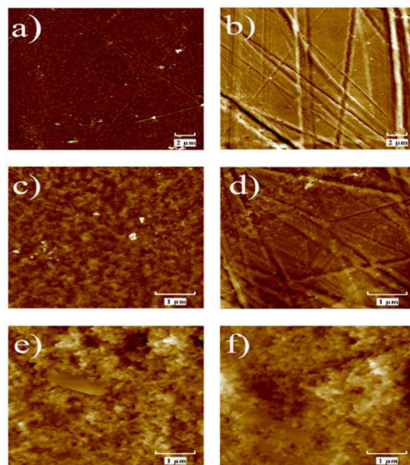
Fig. 1 Surface morphology of plastics substrate and graphite-coated screen-printed electrodes. Representative 20 μm × 20 μm AFM images: (a) Autostat™ polyester z scale = 100 nm; (b) post-consumer PET, z scale = 100 nm. Representative 5 μm × 5 μm AFM images: (c) Autostat™ polyester, z scale = 80 nm; (d) post-consumer PET, z scale = 50 nm; (e) SPE, z scale = 300 nm; (f) PET-SPE, z scale = 500 nm.
