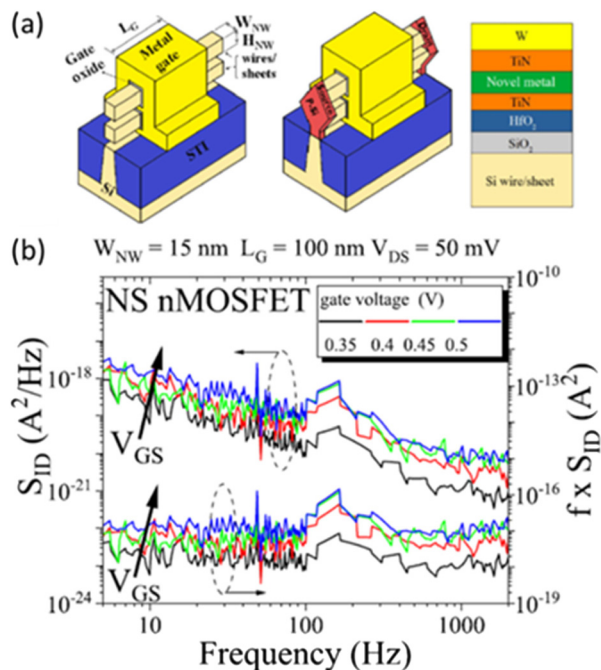
Fig. 24 (a) Schematic diagrams of gate-all-around GAA nFETs with vertically stacked Si nanosheets. (b) Drain current noise power spectral density (left y-axis) and normalized power spectral density (right y-axis) as a function of frequency for a 15 nm nanosheet width device at different gate voltages. Adapted from ref. 72 with permission. Copyright 2020 Institute of Electrical and Electronics Engineers.
