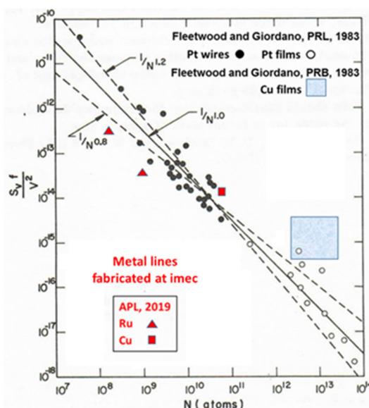
Fig. 9 S_V/V^2 at 295 K and f = 10 Hz for Pt NWs fabricated by substrate step lithography (solid black circles); mechanically scribed, sputtered Pt films (open circles); and mechanically scribed, thermally evaporated Cu films (large, blue box). Lines are proportional to 1/N^{(1.0 \pm 0.2)} . Results are compared with Ru (length L = 10 \mu\text{m} and 50 \mu\text{m} ) and Cu resistors fabricated at imec (small red box). Adapted from ref. 71 with permission. Copyright 2019 American Institute of Physics.
