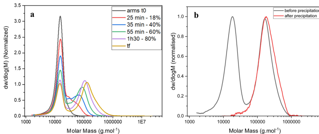
Fig. 2 GPC traces of (a) the kinetic of star formation ( [CL] = 0.2\text{ M} , [CL]/[mCTA] = 3 , [mCTA]/[I] = 20 ) – samples are taken at 0 minute ( t_0 ), 25, 35 and 90 minutes and at the end of the reaction ( t_f – 180 minutes; 95% crosslinker conversion) – the percentage corresponds to the crosslinker conversion measured by ^1\text{H NMR} ; (b) star polymer at t_f and after purification by precipitation, showing complete removal of unreacted arms.
