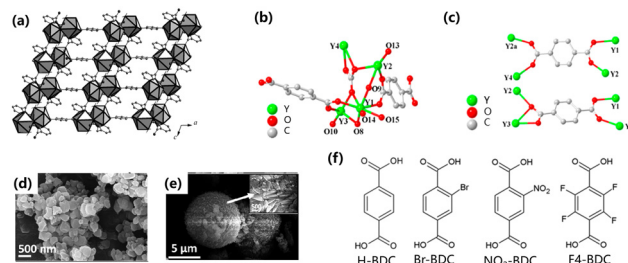
Fig. 1 (a) The 3D structure formed by the connectivity between the 2D layers and BDC linker, Copyright 2008, Wiley VCH. (b) View of the asymmetric unit of Y_{10}(C_8H_4O_4)_6(CO_3)_3(OH)_{12} . (c) View of the coordination mode of BDC ligands, Copyright 2019, American Chemical Society. SEM image of (d) Ce-BDC and (e) Ce-BDC-NH 2 , Copyright 2021, American Chemical Society. (f) Molecular structure of the linkers used. Copyright 2019, American Chemical Society.
