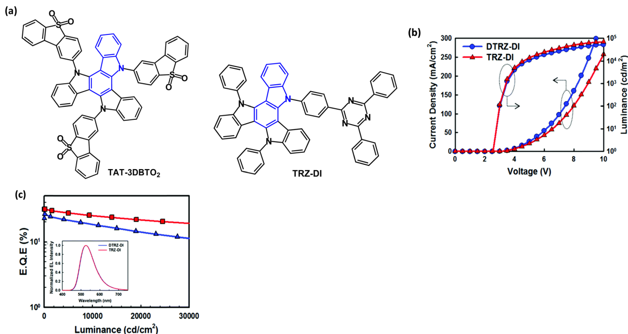
Fig. 24 (a) Molecular structures of TAT-3DBTO 2 and TRZ-DI . (b) Current density–voltage–luminance ( J–V–L ) data. (c) EQE– L data; inset EL spectra for TRZ-DI and DTRZ-DI devices. 140 Copyright 2018 The Royal Society of Chemistry.
