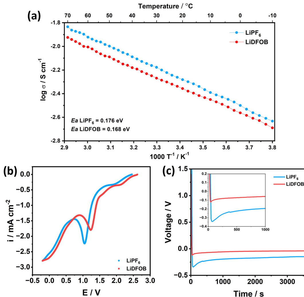
Fig. 2 (a) Arrhenius plot of 1 M LiPF 6 in EC : DEC (1 : 1, v/v) and 1 M LiDFOB in EC : DEC (1 : 1, v/v) electrolyte obtained with electrolyte conductivity measurement from 70 ^{\circ}\text{C} to -10^{\circ}\text{C} . The electrolyte conductivity was measured from -10 to 70 ^{\circ}\text{C} . (b) LSV scan of Li||Cu half cell with 1 M LiPF 6 and 1 M LiDFOB in EC : DEC (1 : 1, v/v) electrolyte with a scan rate of 0.1 \text{ V s}^{-1} . (c) Li plating overpotential at first discharge of Li||Cu half cell with 1 M LiPF 6 and 1 M LiDFOB in EC : DEC (1 : 1, v/v) electrolyte at a current density of 1 \text{ mA cm}^{-2} .
