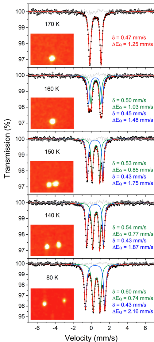
Fig. 2 Mössbauer data of crystalline 1 (toluene-free crystal). Each orange inset shows an equivalent section of the diffraction pattern, corresponding to the (-8 \ -4 \ 6) reflection in the high-temperature indexing in C2/c , and the splitting of the reflection at low temperature is a result of conversion to the twinned structure. Each main panel shows the Mössbauer data (black circles) with the associated fits (red) that are the sum of components for the tetrahedral site (green) and the square-planar site (blue). The residuals are shown in grey.
