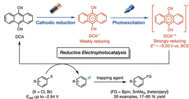
Scheme 6 Reductive electrophotocatalysis with the photoexcited state of DCA - (*DCA - ) for the reductive borylation of aryl chlorides and aryl bromides with bis(pinacolato)diboron (B 2 pin 3 ). Reprinted from ref. 42 with permission from American Chemical Society (Copyright 2010).
