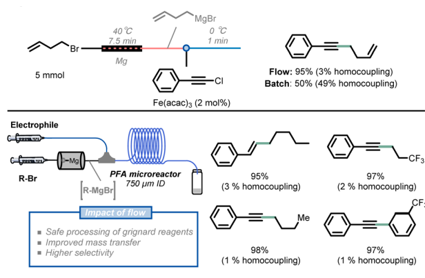
Fig. 5 Combining Grignard reagent synthesis with iron-catalyzed cross-coupling reaction in a telescoped flow process for C(sp) 3 -C(sp 3 ) bond formation.
