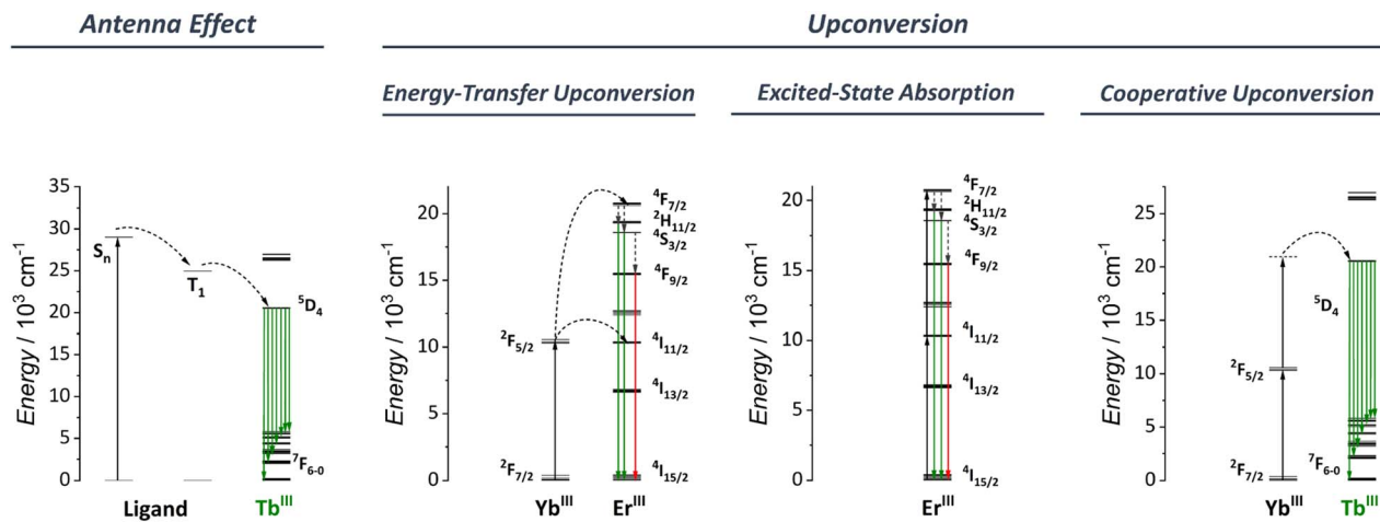
Fig. 3 Depiction of some commonly observed luminescence mechanisms for Ln^{3+} ions. From left to right: Ligand-based antenna effect, Yb^{3+} - Er^{3+} -based energy-transfer upconversion, Er^{3+} -based excited-state absorption, and Yb^{3+} - Tb^{3+} -based cooperative upconversion.
