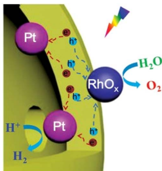
Fig. 9 Schematic of charge separation processes on \text{Pt}@Z\text{nTiO}_{3-x}\text{-N}_y@Rh\text{O}_x . Adapted with permission from ref. 59. Copyright 2021 Wiley-VCH.
