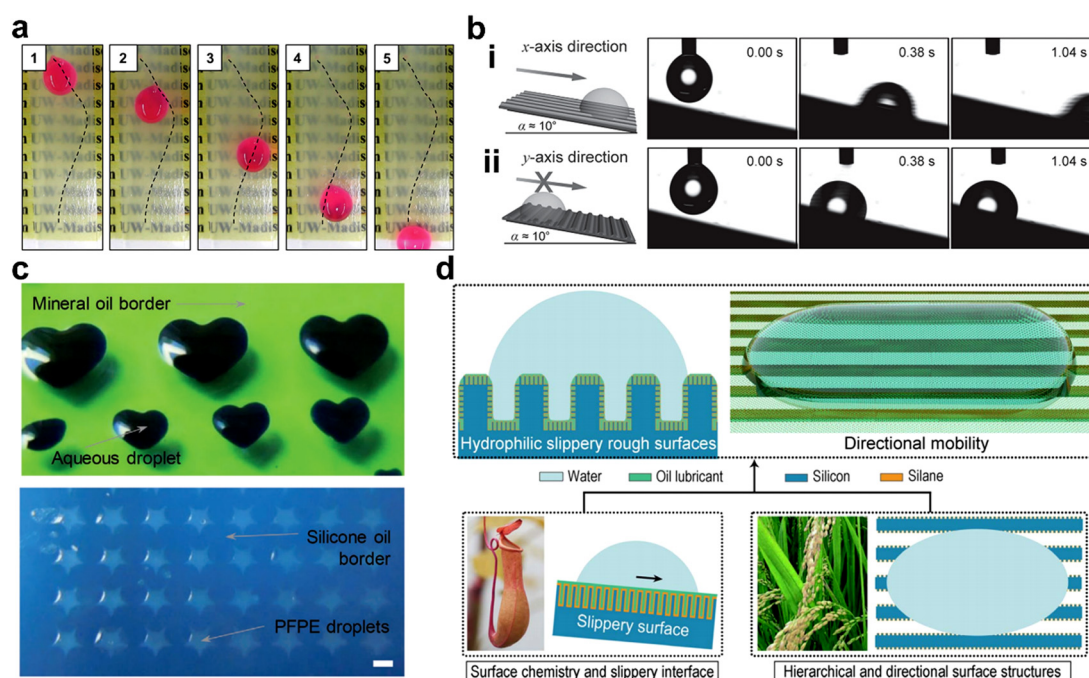
Fig. 7 Droplet manipulation by SLIPSSs with patterns and asymmetric structures. (a) Patterned slippery surface can regulate the sliding pathway of droplets through a selectively hydrophilic modification. 46 (b) Slippery surfaces with a grooved structure achieved an anisotropic droplet manipulation. 15 (c) Images of patterned SLIPSSs with alternative lubricant system including water droplets surrounded by a mineral oil lubricant and perfluoropolyether droplets surrounded by a silicone oil background. 76 (d) SLIPSSs with a directional texture, this structure promotes the coalescence and removal of droplets. 24
