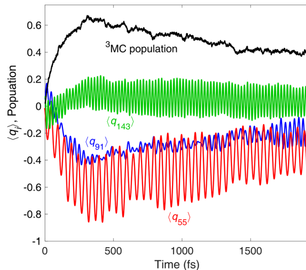
Fig. 7 Average trajectories ( q_{55} ) (red, pyridine ring deformation), ( q_{91} ) (blue, pyridine ring deformation), and ( q_{143} ) (green, internal ligand bending/wagging) of [Fe(bmip) 2 ] 2+ corresponding to three selected ligand modes, as obtained from the simulation with 400 nm excitation. Also shown are the population dynamics of the 3 MC state (black).
