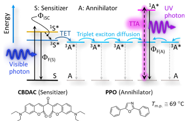
Scheme 1 Schematic energy diagram of TTA-UC in this study. X, ^1X^* , and ^3X^* (X = S: sensitizer or A: annihilator) denote the ground state, excited singlet state, and excited triplet state, respectively. TET: triplet energy transfer; TTA: triplet–triplet annihilation. Bottom shows the sensitizer and annihilator selected in this study.
