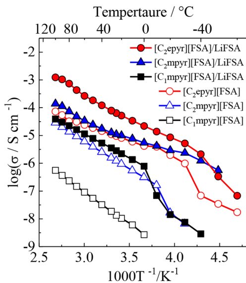
Fig. 3 Arrhenius plots of ionic conductivities for neat pyrrolidinium salts ( 1b ( [C_2\text{mpyr}][\text{FSA}] ), 2b ( [C_1\text{mpyr}][\text{FSA}] ), 3b ( [C_2\text{epyr}][\text{FSA}] )) and 5 mol% LiFSA-doped ones. Reprinted from ref. 43 with permission.
