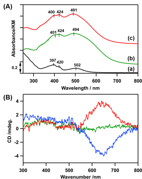
Fig. 1 (A) (a) A transmission UV-vis spectrum of [\text{LCo}_3(\text{NHMe}_2)_6](\text{OTf})_3 in methanol ( c = 0.2 \text{ mol L}^{-1} ). (b) and (c) DR UV-vis spectra of (b) \text{LCo}_3/\text{en-SiO}_2 , and (c) \text{LCo}_3((R)\text{-A1})/\text{en-SiO}_2 . (B) DR CD spectra of \text{LCo}_3/\text{en-SiO}_2 (green), \text{LCo}_3((R)\text{-A1})/\text{en-SiO}_2 (red) and \text{LCo}_3((S)\text{-A1})/\text{en-SiO}_2 (blue).
