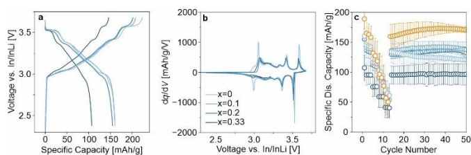
Fig. 4 (a) First-cycle charge-discharge curves of SSB cells using LRLNO 0-750, 0.1-750, 0.2-750, or 0.33-750 at 45 °C and at 0.1C rate. (b) Second-cycle differential capacity curves. (c) C-rate testing at 0.1C (one cycle), 0.2C, 0.5C, 1C, and 2C (three cycles each) followed by cycling at 0.2C. The orange data points display the performance of LNO with a cobalt-based coating. The error bars represent the standard deviation from three independent cells.
