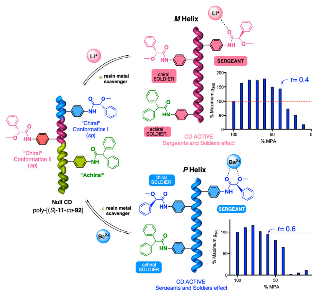
Fig. 39 On/Off Sergeants and Soldiers effect in poly-[ 11 - co - 92 1- n ] copolymer series by metal ions (on) and resin metal scavengers (off). Reproduced from ref. 227 with permission from the Royal Society of Chemistry, copyright 2014.
