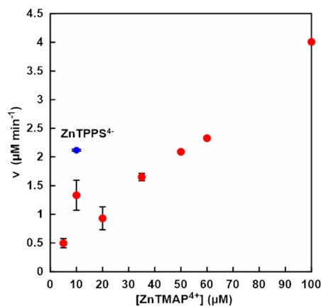
Fig. 3 The concentration of ZnTMAP 4+ dependence of NADH production rate (v) with the system of TEOA, ZnTMAP 4+ , [Cp*Rh(bpy)(H 2 O)] 2+ and NAD + in 5.0 mL of 500 mM HEPES buffer (pH 7.8). Blue circle shows the NADH production rate (v) with the system of TEOA, ZnTPPS 4- , [Cp*Rh(bpy)(H 2 O)] 2+ and NAD + in 5.0 mL of 500 mM HEPES buffer (pH 7.8). Errors were obtained from the average of multiple trials.
