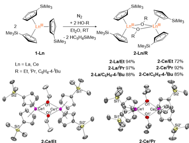
Fig. 2 Top: synthesis of 2-Ln/R by alcoholysis of 1-Ln in \text{Et}_2\text{O} . Bottom: crystal structures of 2-Ce/Et and 2-Ce/ i Pr with displacement ellipsoids at the 50% probability level. Hydrogen atoms and disorder were removed for clarity.
