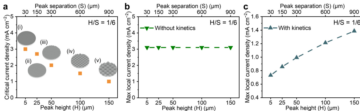
Fig. 2 Experimentally determined critical currents for dendrites and calculated maximum current densities for egg-box contoured surfaces with the same ratio of peak height ( H ) to separation ( S ). (a) Experimentally determined critical current densities for all five constant H/S ratio surfaces (orange squares), the 3D simulated surfaces for each are also shown in grey (i) H5S30 (ii) H25S150 (iii) H50S300 (iv) H100S600 (v) H150S900. (b) Calculated maximum (max) local current density without including Li deposition kinetics for all five constant H/S ratio surfaces for 1 \text{ mA cm}^{-2} geometrical current density. (c) Calculated maximum (max) local current density including Li deposition kinetics for all five constant H/S ratio surfaces for 1 \text{ mA cm}^{-2} geometrical current density.
