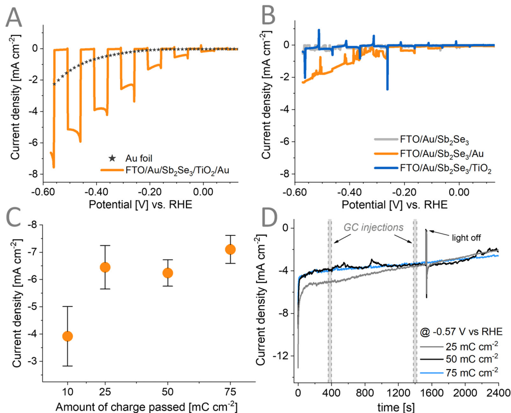
Fig. 6 Linear sweep photovoltammogram under 1 sun illumination ( AM1.5G , 100 \text{ mW cm}^{-2} ) of (A) the complete architecture (Au catalyst loading of 75 \text{ mC cm}^{-2} deposited at -0.25 \text{ V vs. Ag/AgCl} ) and (B) the set of incomplete electrode architectures in a \text{CO}_2 -saturated solution of 0.5 \text{ M KHCO}_3 . (C) Recorded current density at -0.57 \text{ V vs. RHE} for different catalyst loadings deposited at -0.25 \text{ V vs. Ag/AgCl} . (D) Long-term chronoamperometry measurement of the architecture with different catalyst loadings deposited at -0.25 \text{ V vs. Ag/AgCl} .
