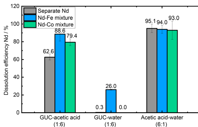
Fig. 4 The dissolution efficiency of \text{Nd}_2\text{O}_3 from separate \text{Nd}_2\text{O}_3 leaching (grey), 1 : 1 (wt%) \text{Nd}_2\text{O}_3 : \text{Fe}_2\text{O}_3 mixture (blue), and 1 : 1 (wt%) \text{Nd}_2\text{O}_3 : \text{Co}_3\text{O}_4 mixture (green) in GUC–acetic acid (1 : 6), GUC–water (1 : 6), and acetic acid–water (6 : 1). A 10 mg of oxide sample was dissolved in a 1.5 mL of solvent at 50 °C for 24 h with a stirring speed of 500 rpm.
