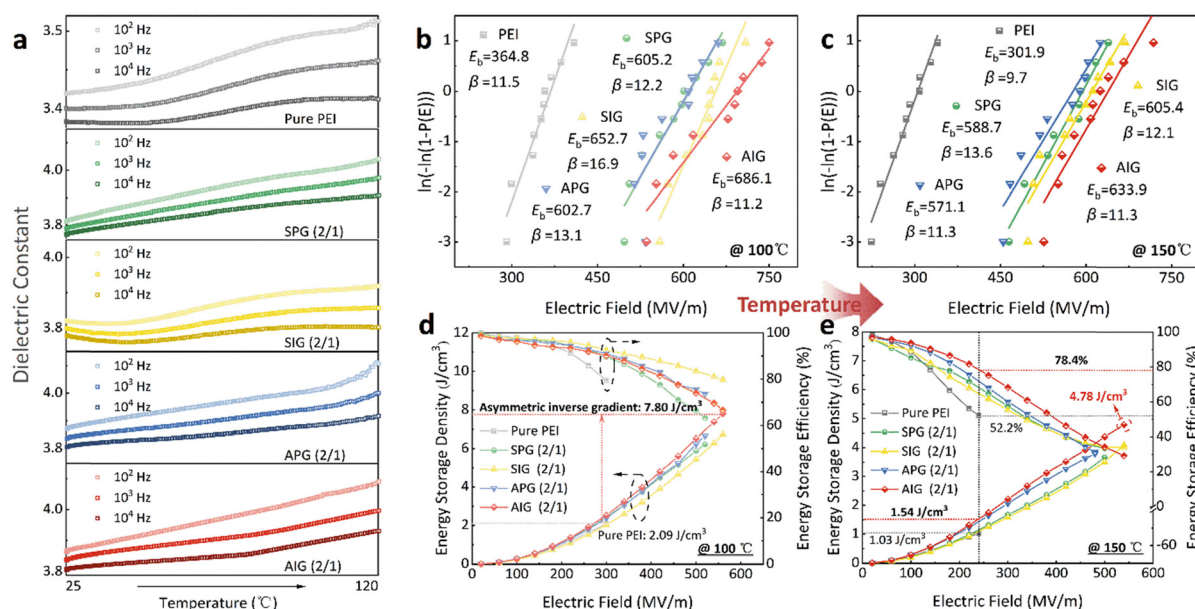
Fig. 7 (a) The temperature dependence of the dielectric constant of pure PEI, and SPG (2/1), SIG (2/1), APG (2/1), and AIG (2/1) composite dielectrics at 10^2 , 10^3 , and 10^4 Hz. The breakdown strength of pure PEI, and SPG (2/1), SIG (2/1), APG (2/1), and AIG (2/1) composite dielectrics at (b) 100 °C and (c) 150 °C. The energy storage density and efficiency of pure PEI, and SPG (2/1), SIG (2/1), APG (2/1), and AIG (2/1) composite dielectrics at (d) 100 °C and (e) 150 °C.
