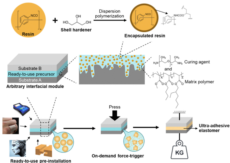
Fig. 1 Illustration of the on-demand ultra-high adhesion formation of the ready-to-use precursor and its preparation process. The resin, curing agent, and matrix polymer are MDI- prepolymer, PPG-diamine, and acrylates copolymer, respectively.
