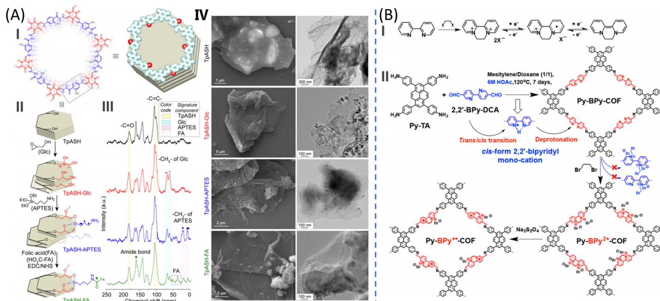
Fig. 6 Post-synthetic modification (PSM). (A) I. A schematic diagram of the chemical structure of COF nanosheets. II. Sequential PSM processes of TpASH to TpASH-Glc and their NMR spectra (III), as well as SEM and TEM images (IV). Reproduced from ref. 48 with permission from Journal of the American Chemical Society, Copyright 2017. (B) I. Two reversible redox states of a bipyridine-like structure. II. Sequential PSM processes of Py-BPy-COF to Py-BPy 2+ -COF or Py-BPy •+ -COF. Reproduced from ref. 49 with permission from Journal of the American Chemical Society, Copyright 2019.
