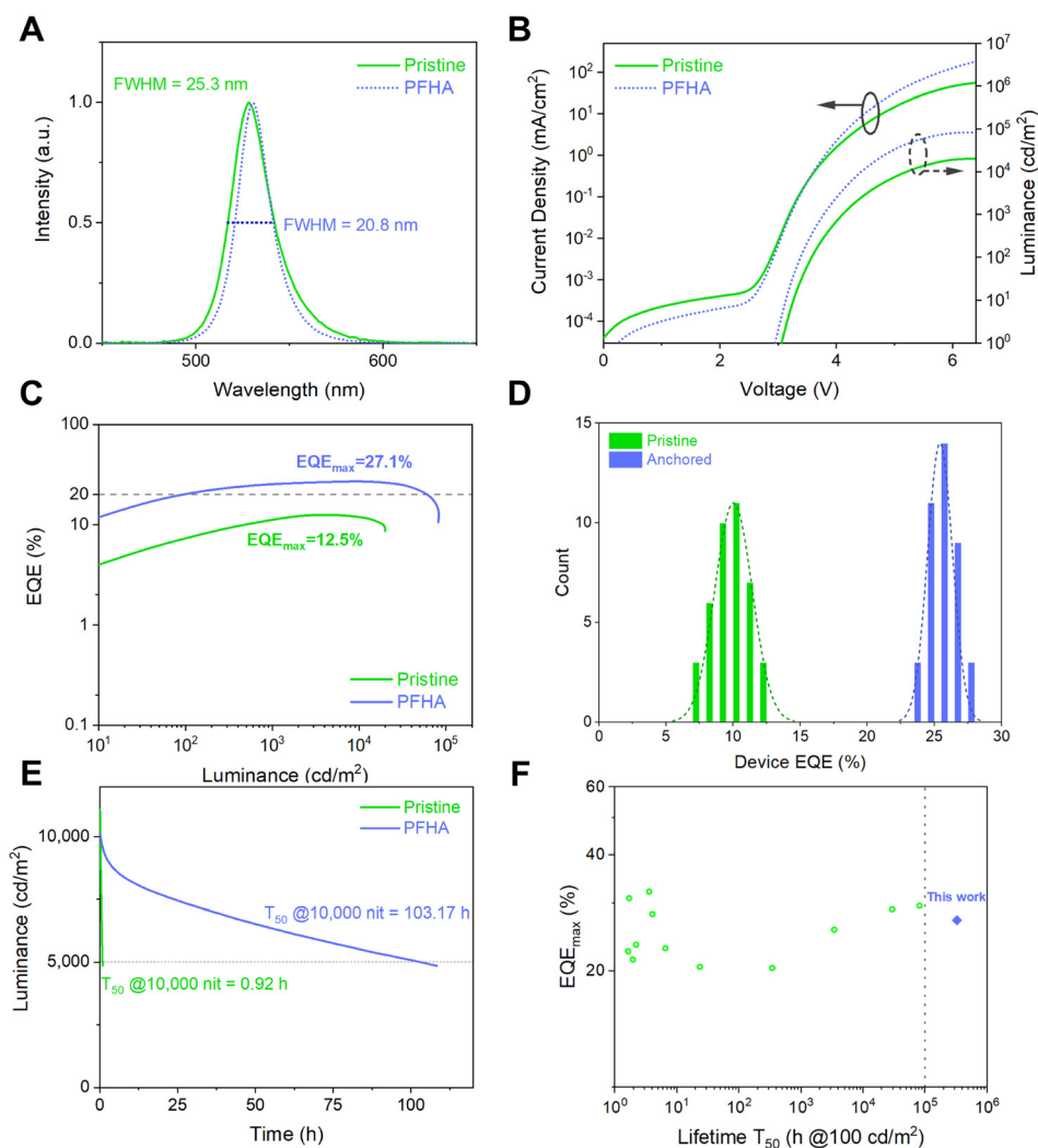
Fig. 4 Ultra-stable and efficient PeLEDs. (A) EL spectra and (B) J – V – L plots of a representative PeLED device. (C) EQE to luminance curve of PeLEDs. (D) Statistical device EQE_{max} of pristine and PFHA PeLEDs. 40 devices are measured in total. (E) Operational lifetime of pristine and PFHA-anchored PeLED devices. (F) Summary of the reported PeLED performance based on the maximum EQE and estimated or measured T_{50} at 100 cd m -2 .
